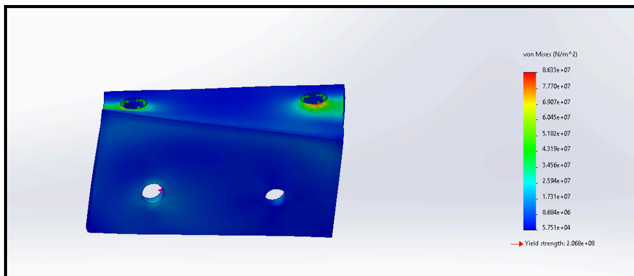
Figure 5.7: Stage 1 Chain Bracket
