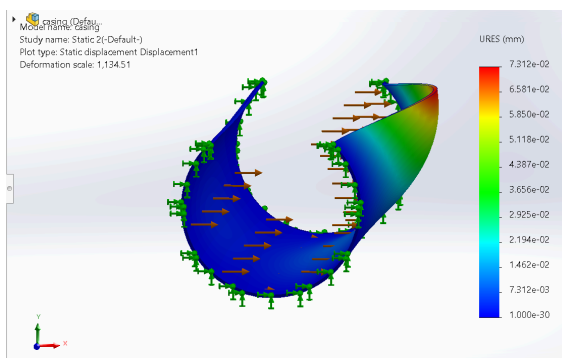
Figure 2.3: FEA results from side orientation of deflection
