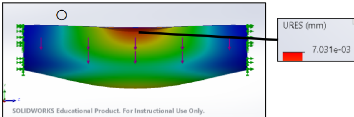
Figure 2.2: FEA results from upright orientation of deflection
