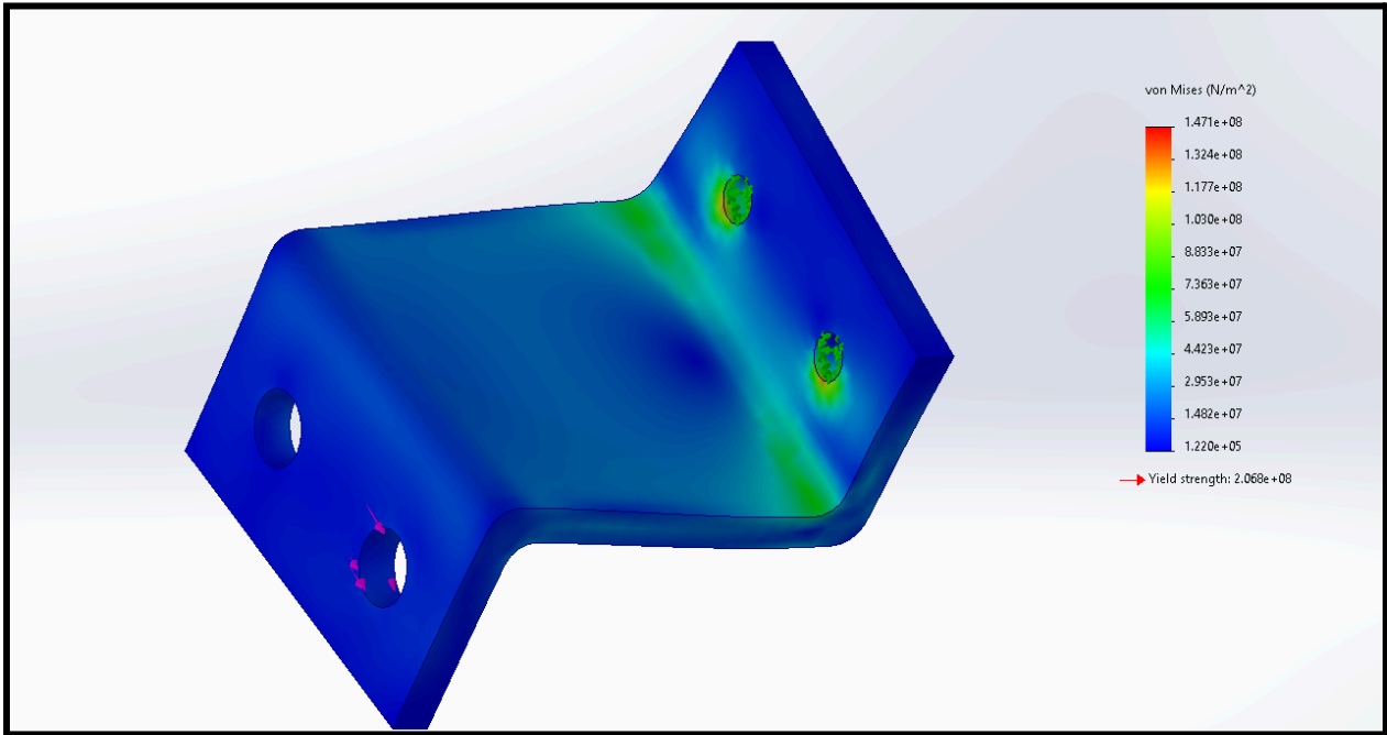
Figure 5.6: Stage 0 Chain Bracket
