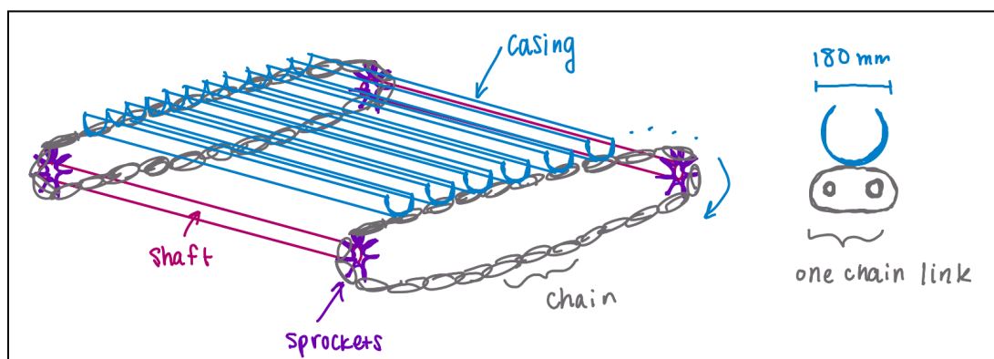
Figure 1.4. Conceptual drawing of chain loader with a unit link shown on the side
