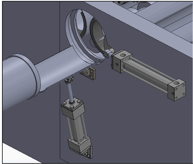
Figure 4.9, Blast Door and Rail Open
