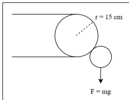
Figure 3.0: System Model for Torque Calculation
