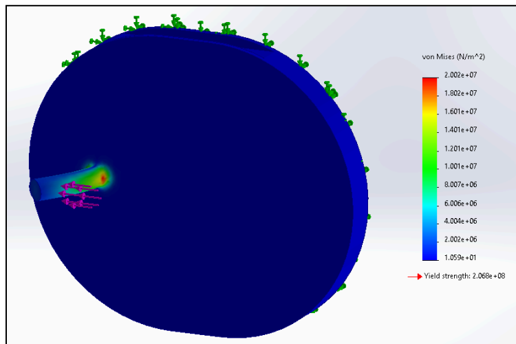
Figure 4.7, Blast Door FEA
