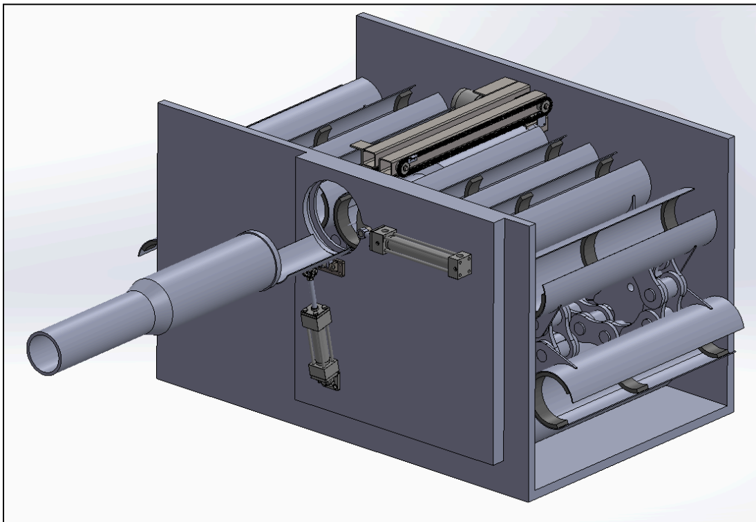
Figure 6.1: Full Assembly Model
