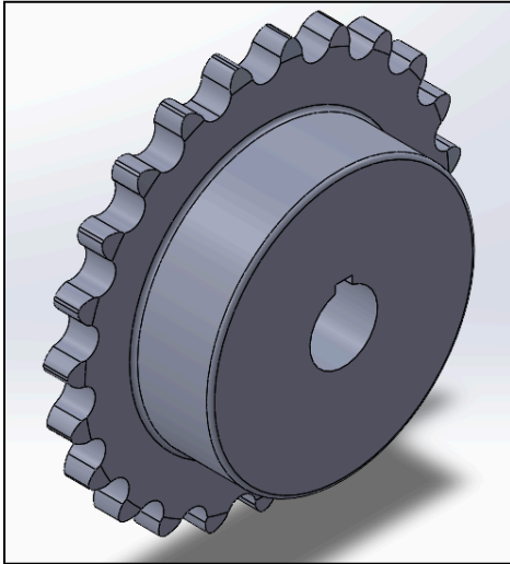
Figure 3.2: 12B23 Sprocket
