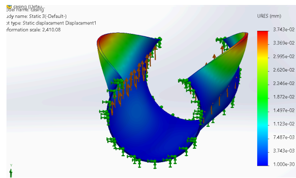
Figure 2.4: FEA results from bottom orientation of deflection
