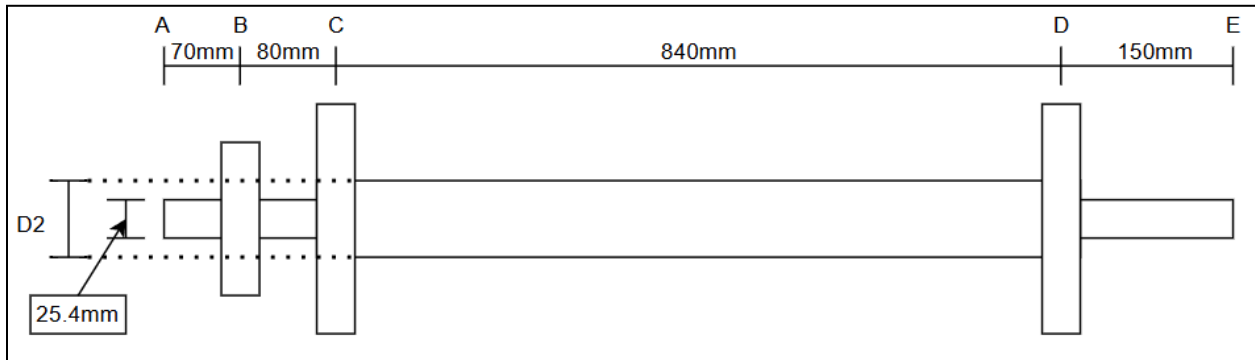
Figure 3.5: Driven Shaft Analytical Model
