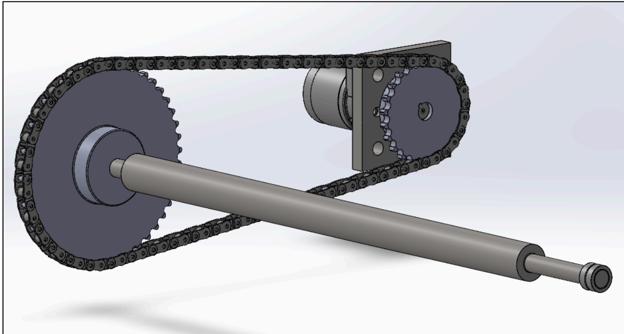
Figure 3.9: Power Transmission Final Design
