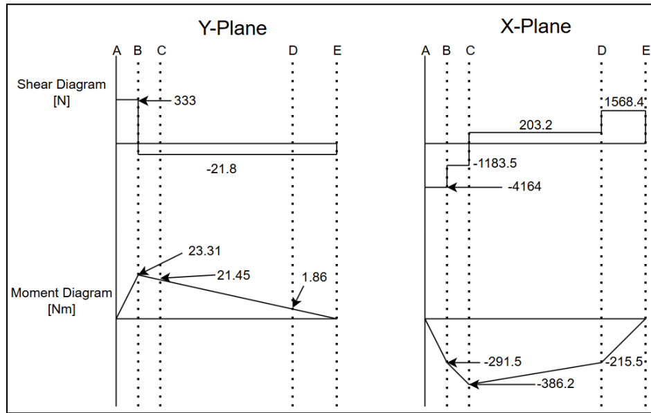
Figure 3.6: Driven Shaft Shear and Moment Diagrams
