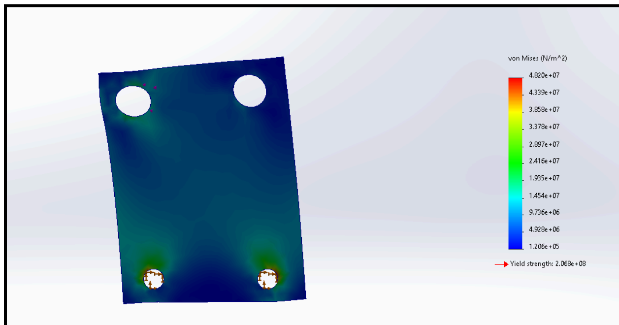
Figure 5.8: Stage 2 Chain Bracket
