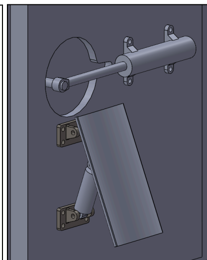
Figure 4.4, Double Hydraulic Cylinder Design Model
