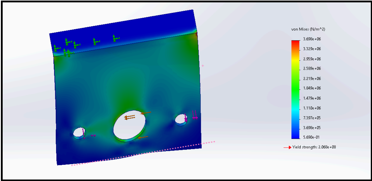
Figure 5.5: Motor Mount
