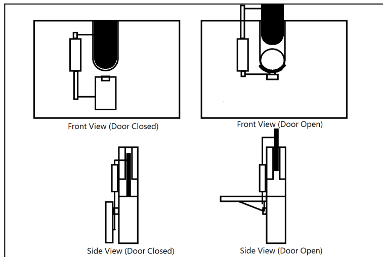
Figure 4.1, Single Hydraulic Cylinder Design
