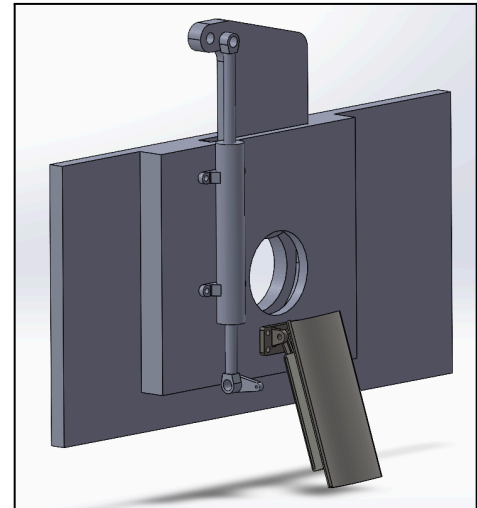
Figure 4.2, Single Hydraulic Cylinder Design Model
