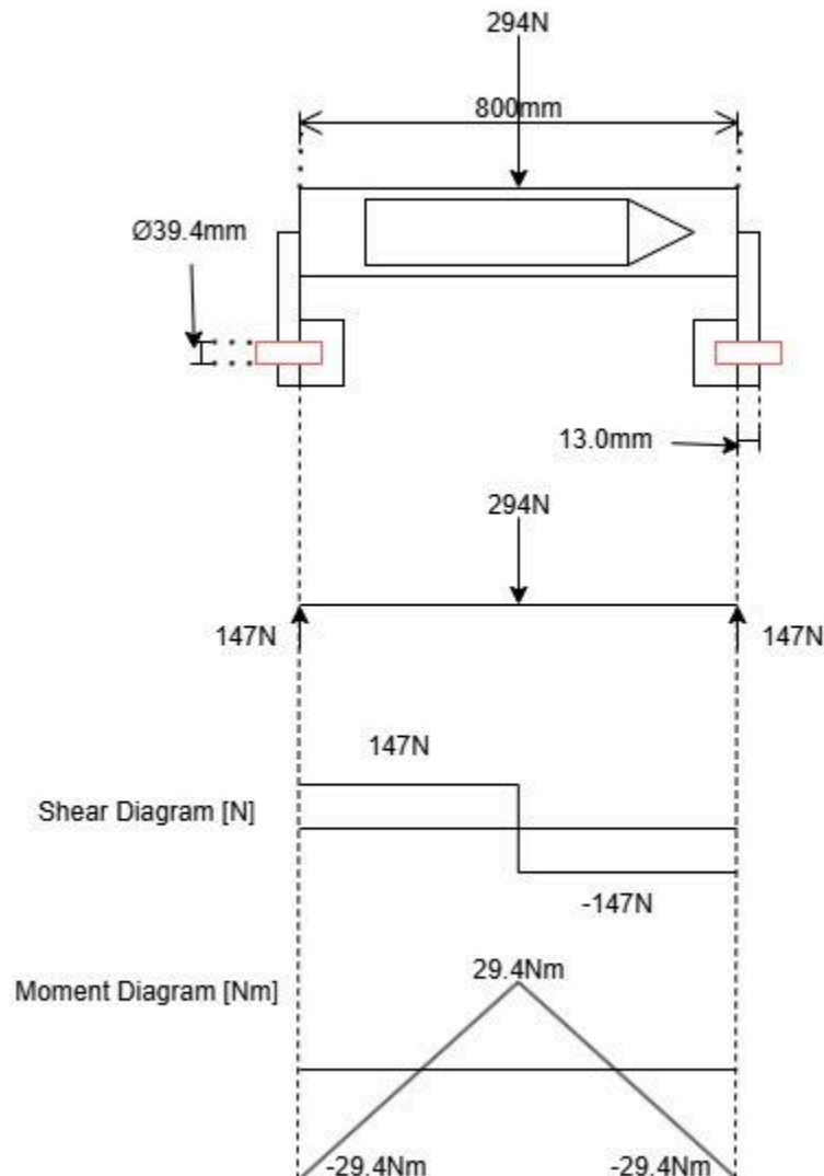
Figure 2.7: Illustration of beam with shear and moment deflection analysis
