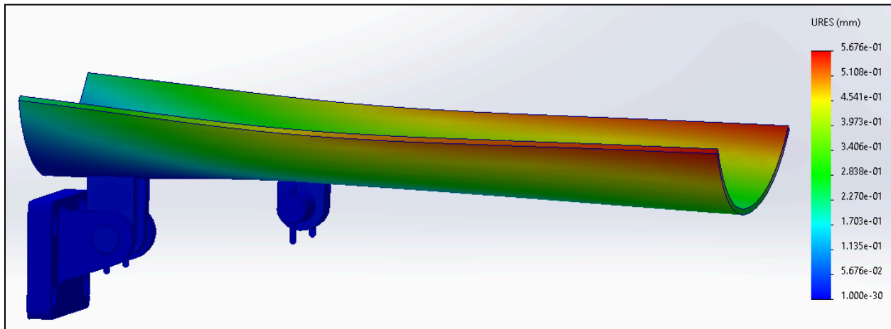
Figure 4.5, Rail Deflection FEA
